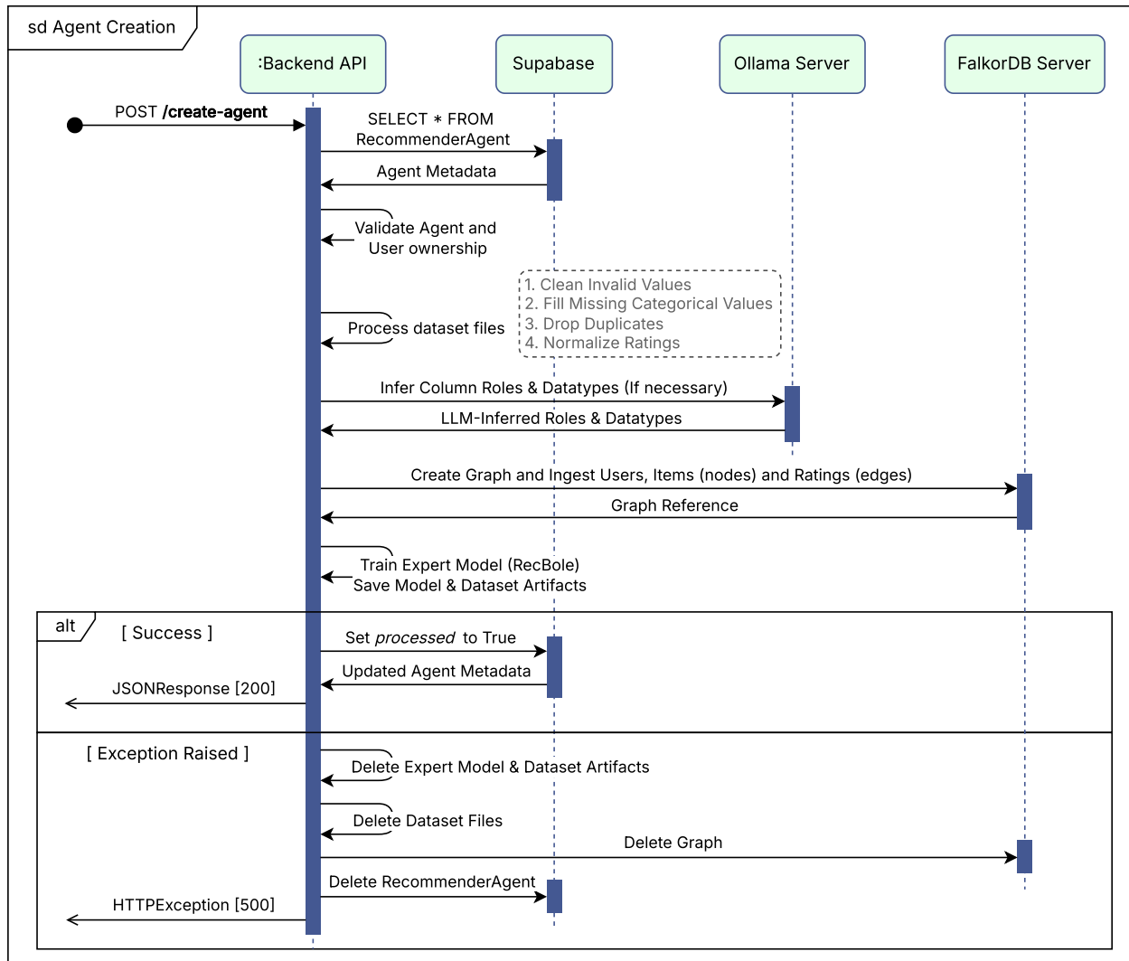
Figure 3.4: Sequence Diagram for Agent Creation.
