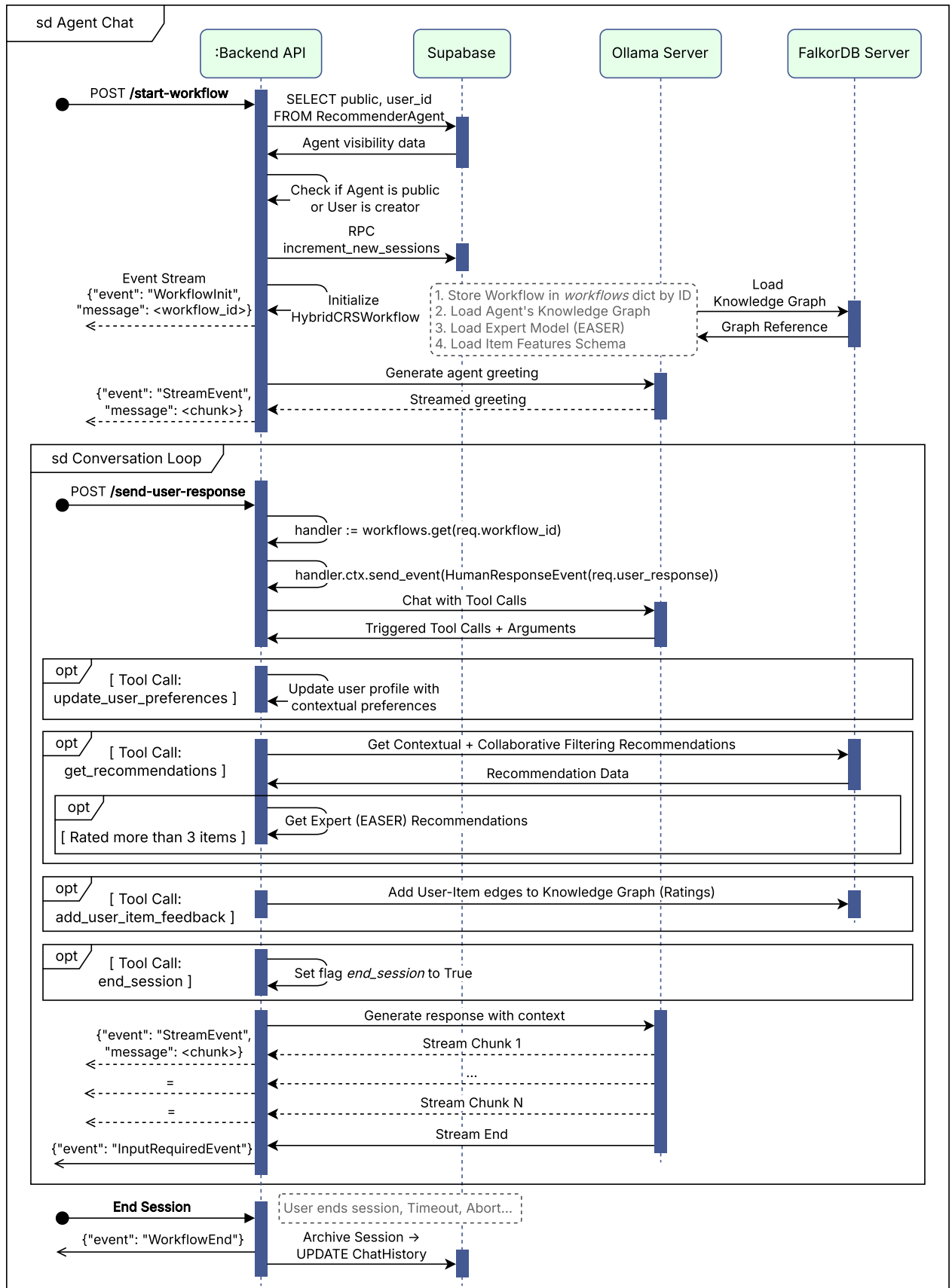
Figure 3.5: Sequence Diagram for an Agent Chat interaction.
