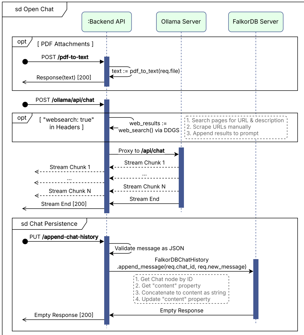
Figure 3.6: Sequence Diagram for an Open Chat interaction.
