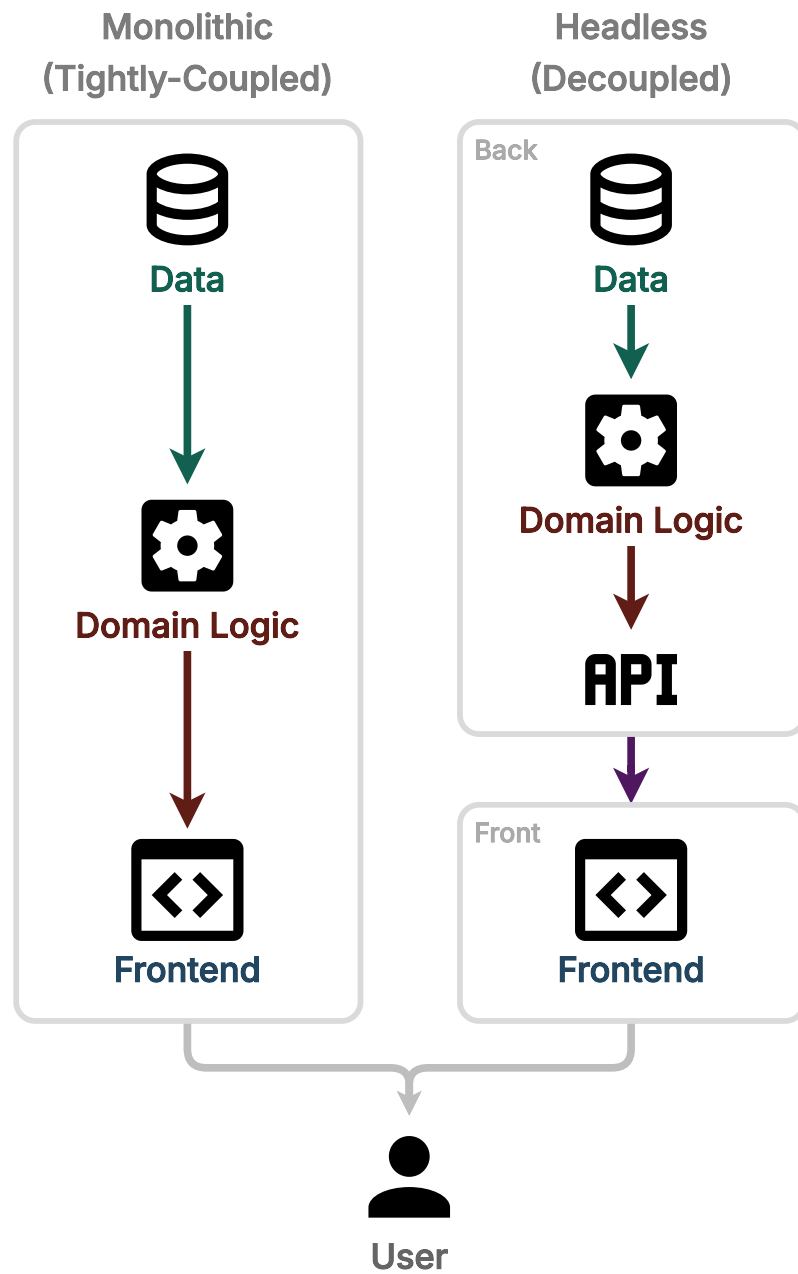
Figure 2.2: Comparison between Monolithic and Headless web architectures.
