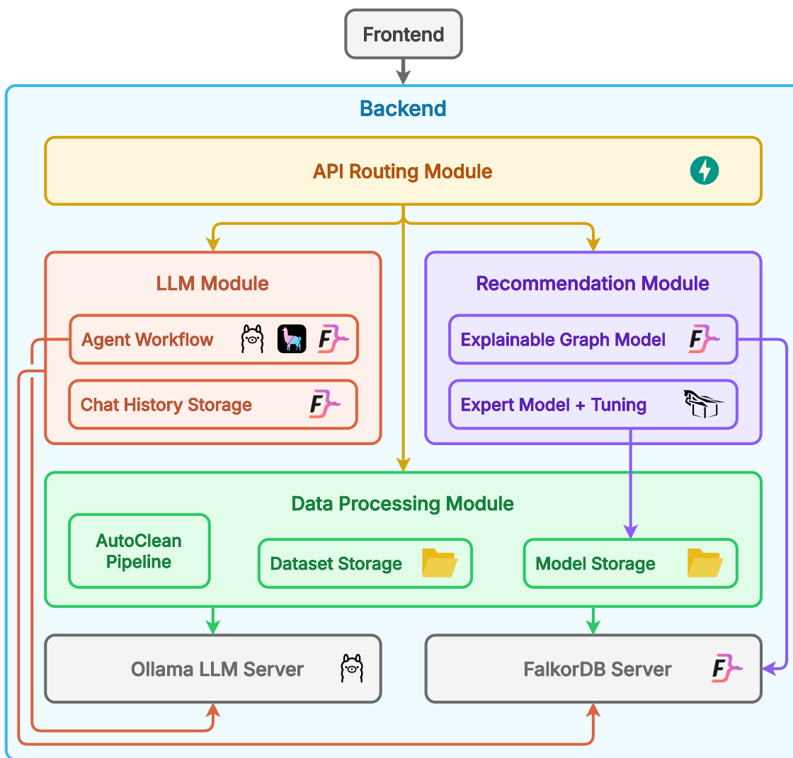
Figure 3.3: Backend Module Diagram.
