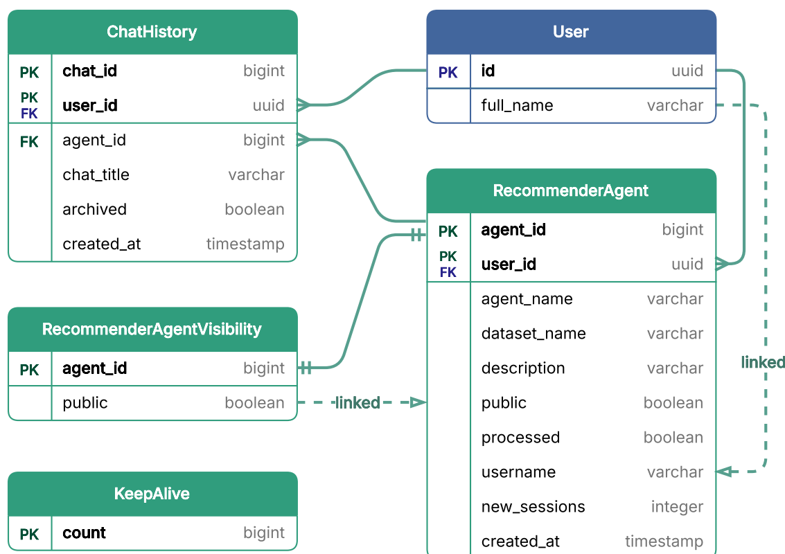
Figure 3.7: ER Diagram for the Metadata Database.
