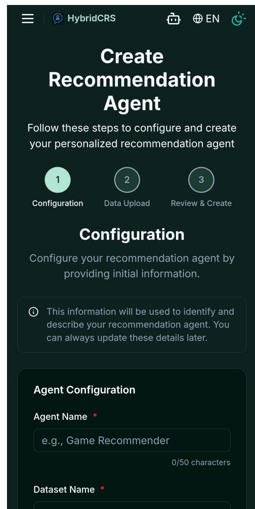
(b) Create Agent
