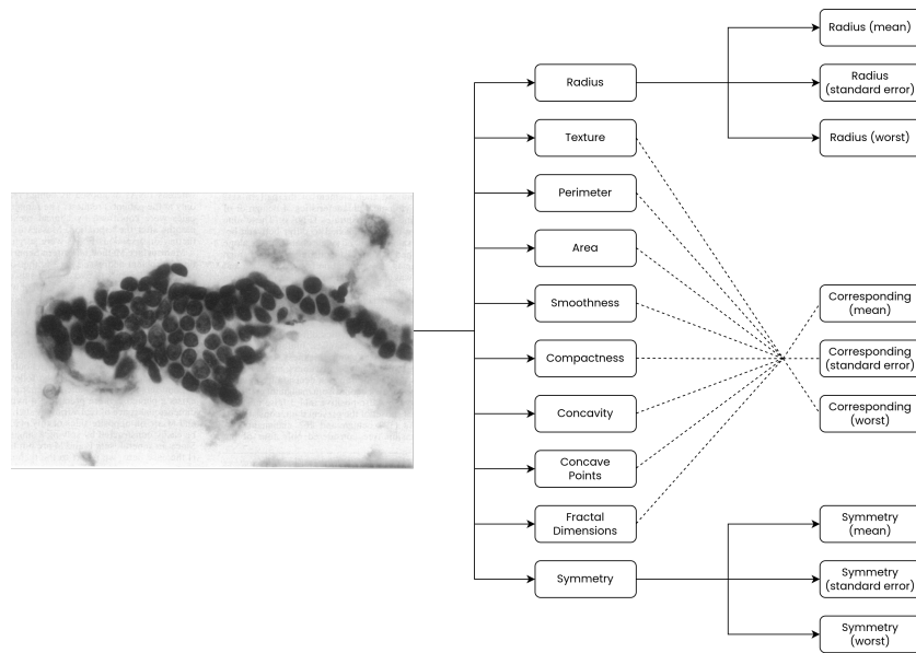
Figure 3.3: Features of the Breast Cancer Wisconsin dataset, FNAB sample picture taken from [33], the rest of the diagram is original.
