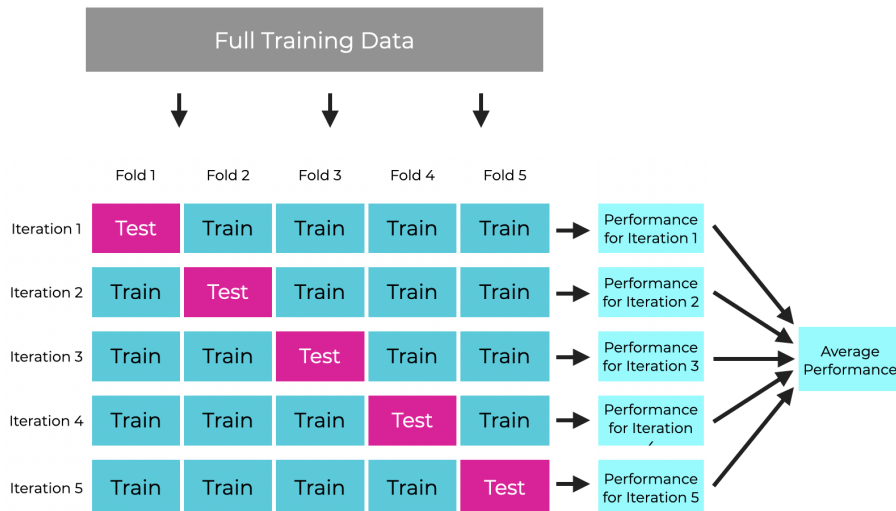
Figure 2.6: Graphical representation of a 5 fold CV [24].
