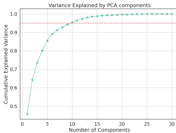
Figure 3.5: Cumulative explained variance when using PCA.
