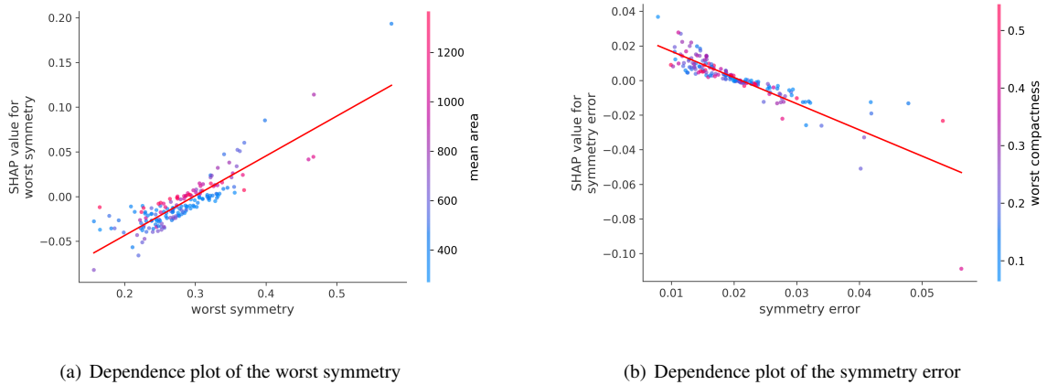
Figure 4.9: Dependence plots of the worst symmetry and the symmetry error using the Logistic Regression classifier.
