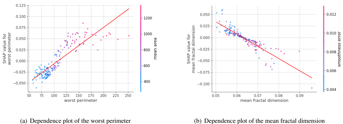
Figure 4.6: Dependence plots of the Worst Perimeter and the Mean Fractal Dimension using the Logistic Regression classifier.
