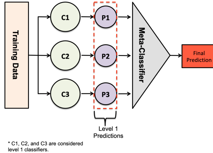
Figure 2.4: Graphical representation of Stacking [19].
