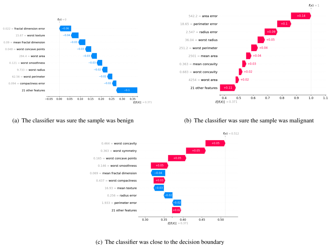
Figure 4.7: Waterfall plots of the Logistic Regression classifier.
