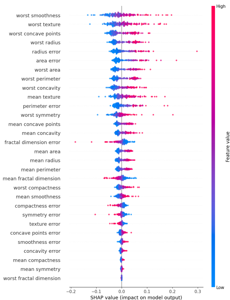
Figure 4.5: Beeswarm plot of the Logistic Regression classifier.
