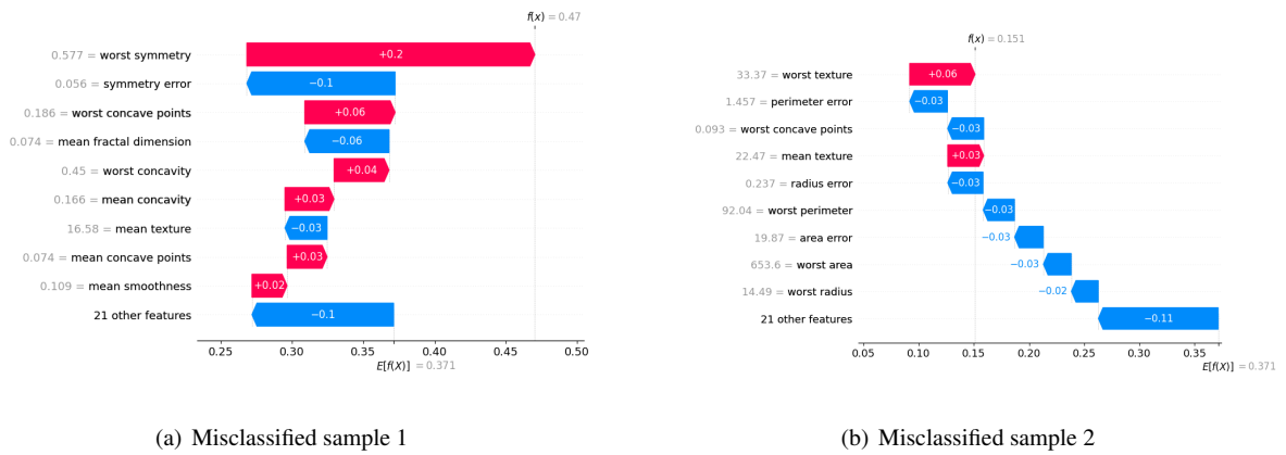
Figure 4.8: Waterfall plot of the two samples that were misclassified by the Logistic Regression classifier.
