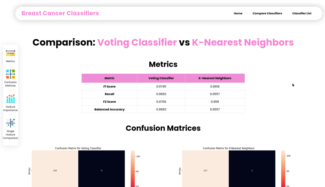
Figure B.2: Comparison of two classifiers.
