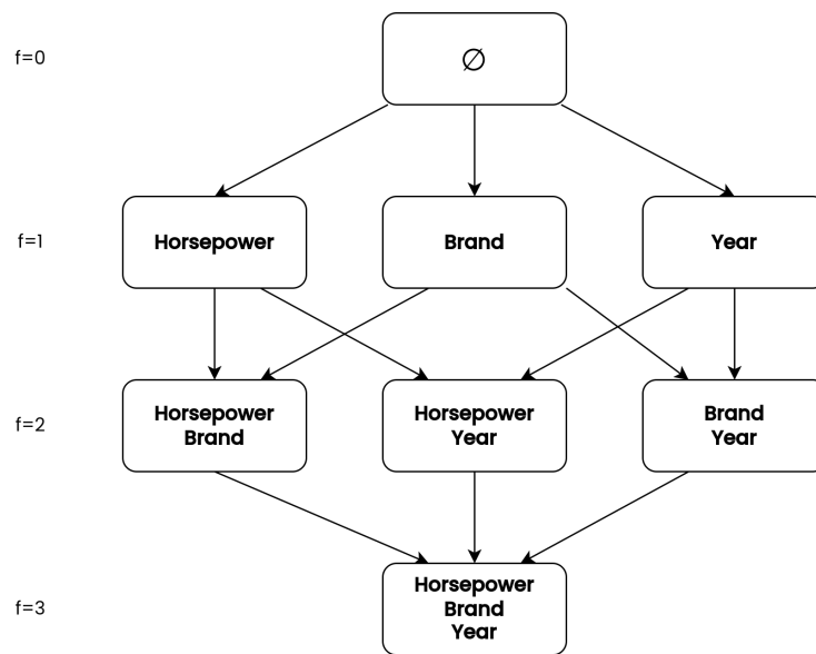
Figure 2.7: Powerset with the features of the car example.
