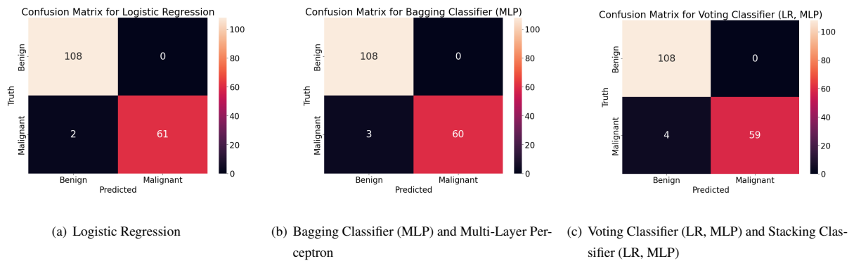
Figure 4.4: Confusion matrices of the five best classifiers.
