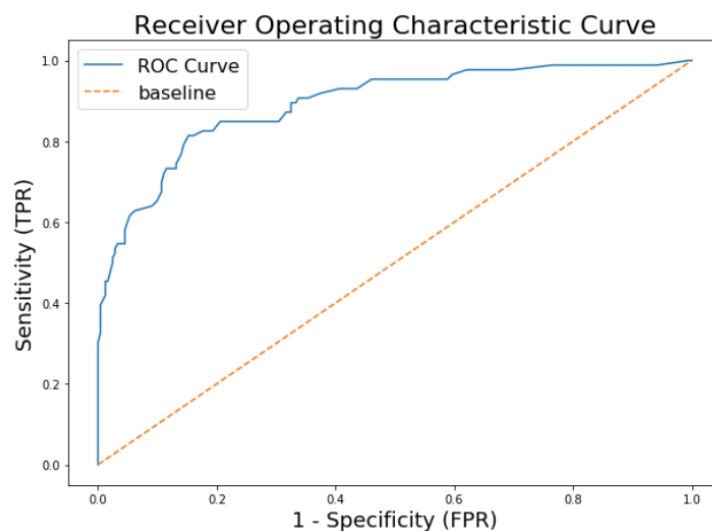
Figure 2.5: Example of a ROC Curve, the y-axis is the True Positive Rate or Recall, and the x-axis is the FP Rate [23].
