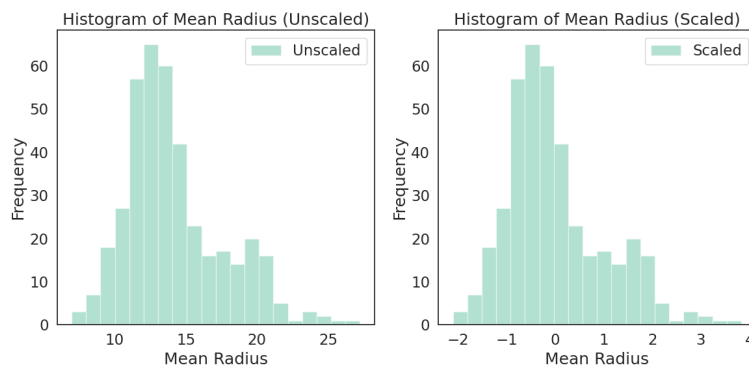
Figure 3.4: Standardization before and after of mean radius.
