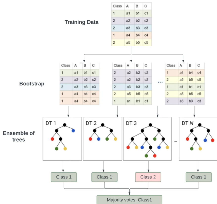
Figure 2.2: Graphical representation of Random Forest [14].
