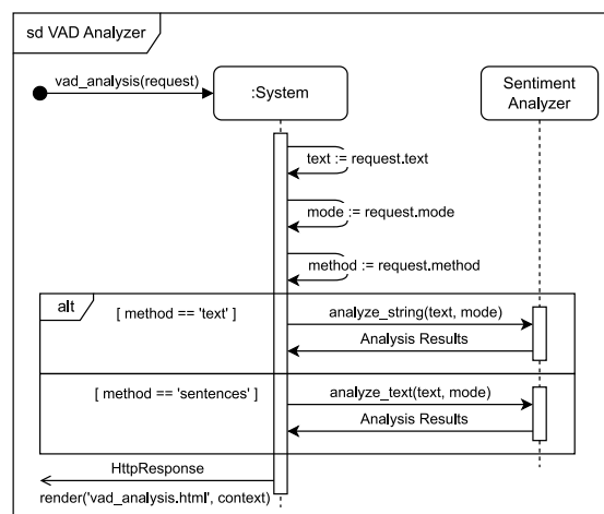
Figure 3.3: Sequence diagram: VAD Analyzer
