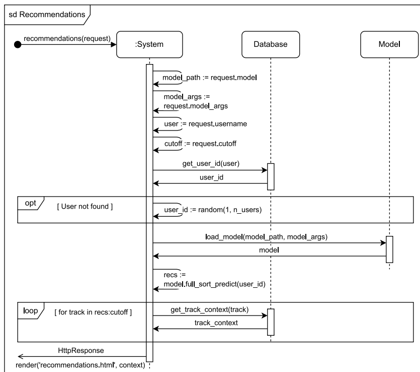
Figure 3.5: Sequence diagram: Recommendations
