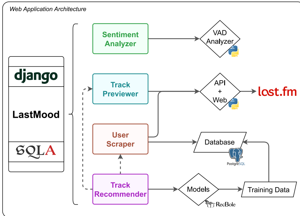
Figure 3.1: Web application architecture
