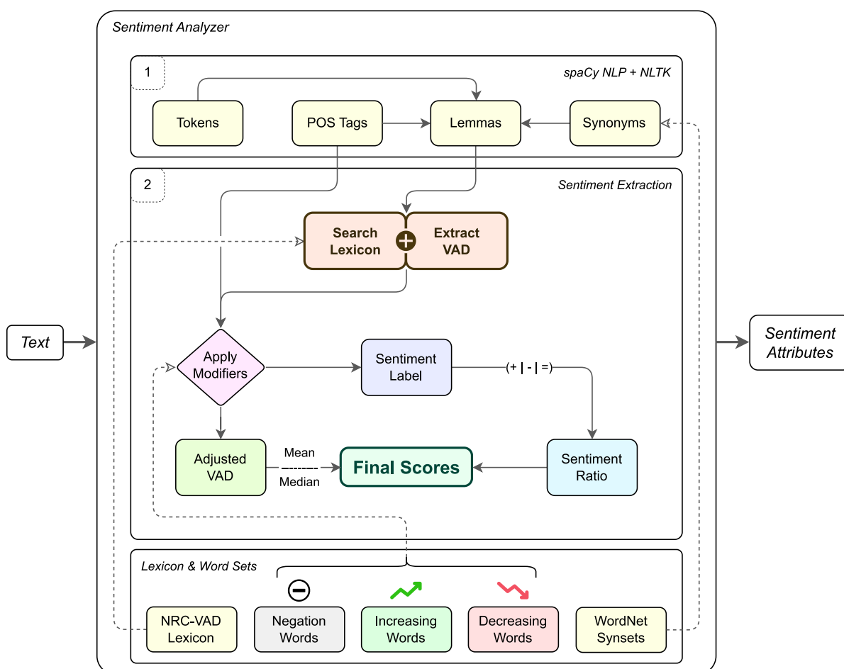
Figure 3.11: Sentiment analyzer structure
