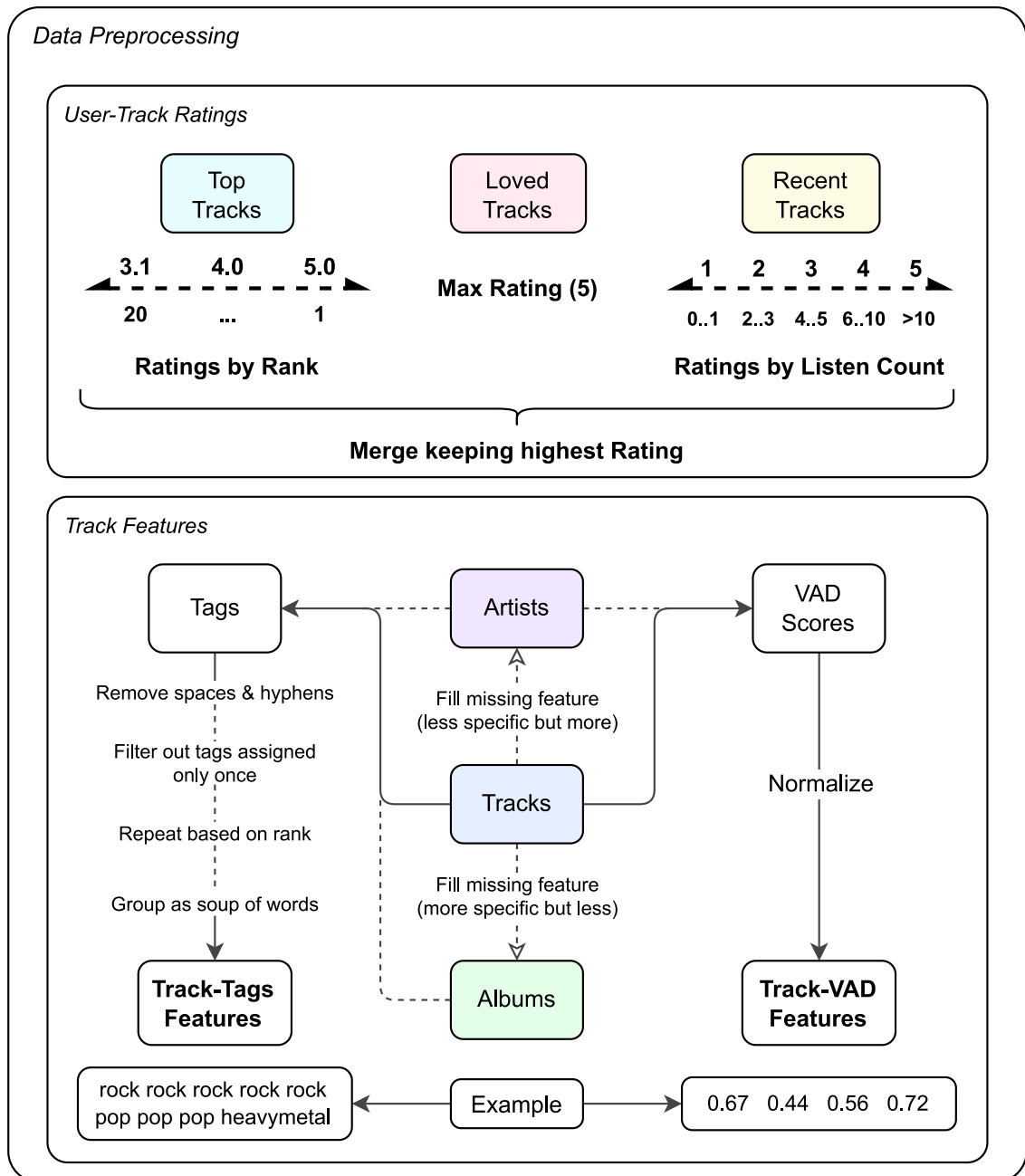
Figure C.1: Data Preprocessing
