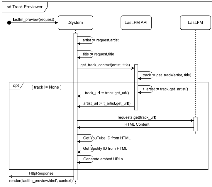
Figure 3.2: Sequence diagram: Track Previewer
