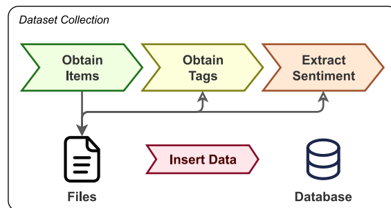
Figure 3.7: Dataset collection
