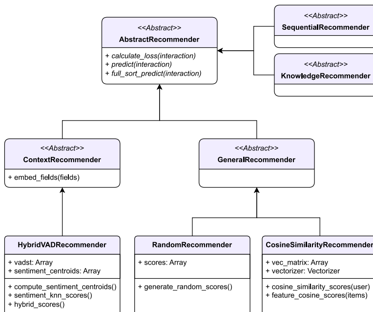
Figure 3.6: Class diagram: Recommendation models
