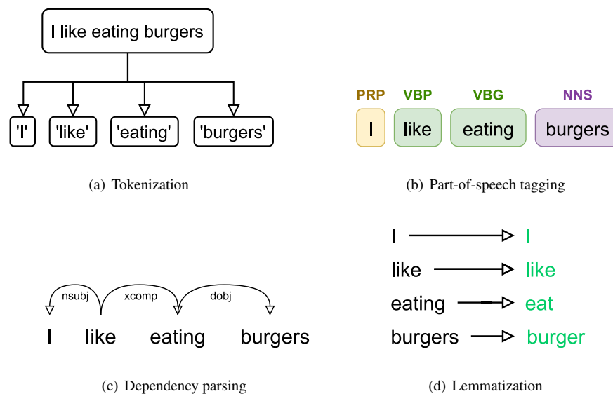
Figure 2.1: Text processing techniques
