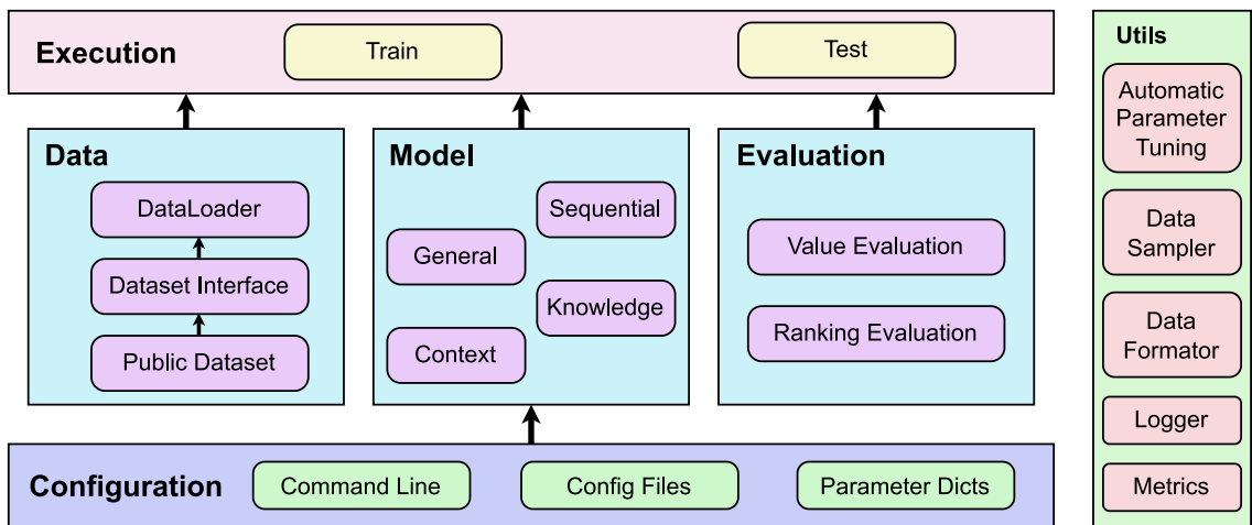
Figure B.1: RecBole Framework [19]
