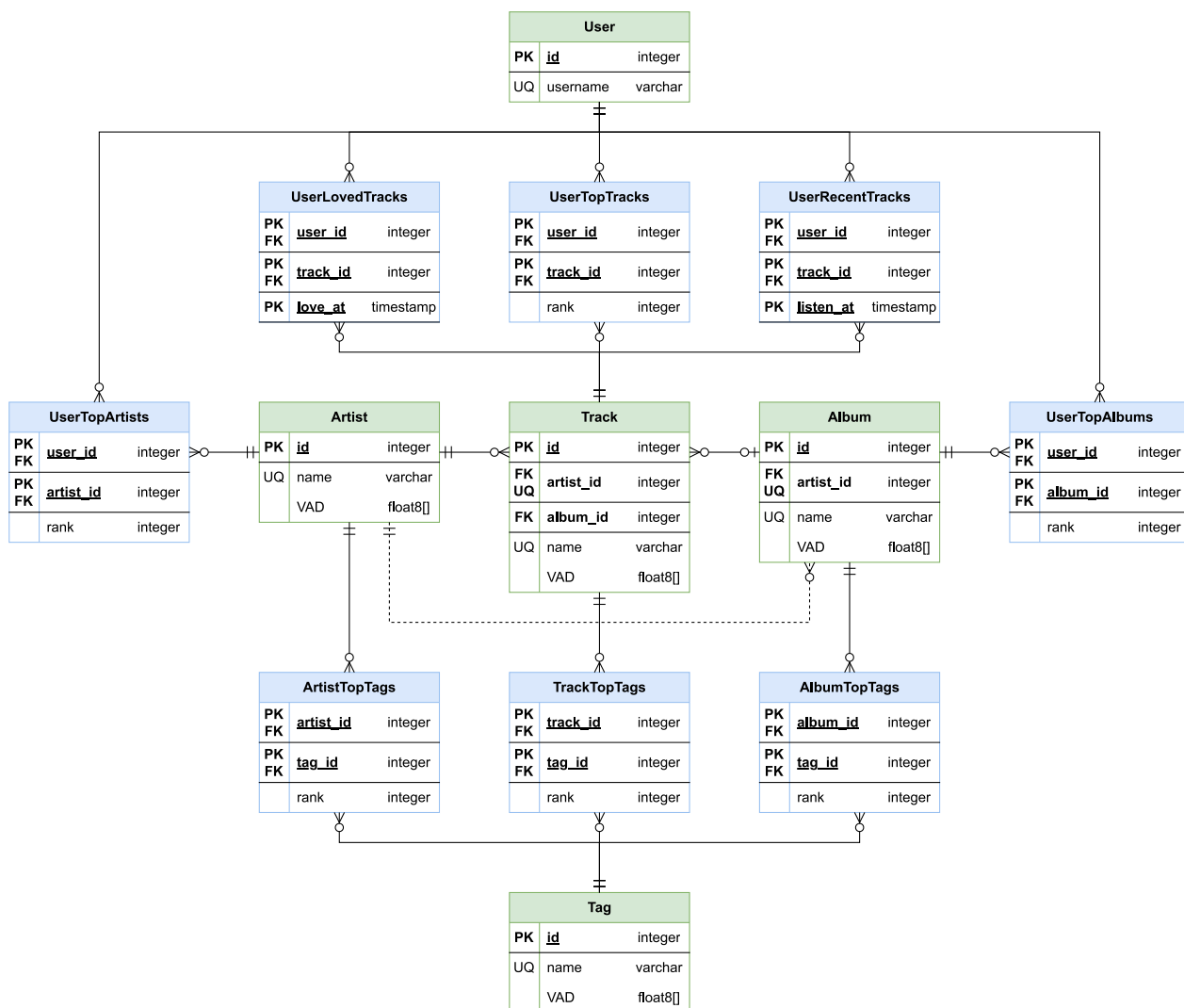
Figure 3.8: Entity-Relationship diagram of the Last.fm scraped database, where PK, FK and UQ mean primary key, foreign key & unique, respectively.
