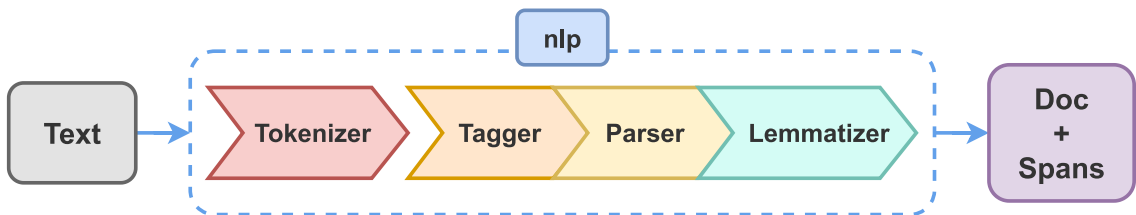
Figure B.2: spaCy NLP Pipeline
