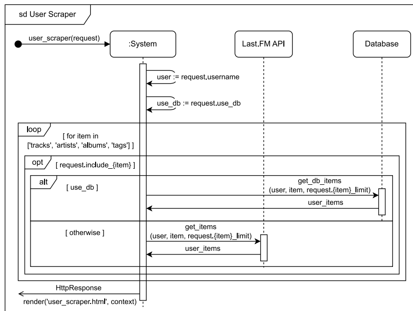
Figure 3.4: Sequence diagram: User Scraper
